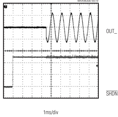
SHUTDOWN WAVEFORM
