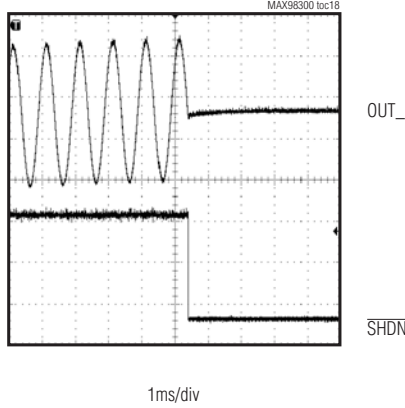
STARTUP WAVEFORM
