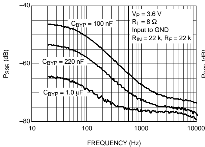
Figure 12. P_{SSR} versus Frequency and C_{BYP} @ V_P = 3.6 V, A_V = 2
