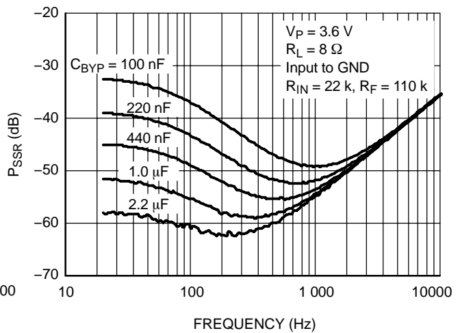
Figure 13. P_{SSR} versus Frequency and C_{BYP} @ V_P = 3.6 V, A_V = 10
