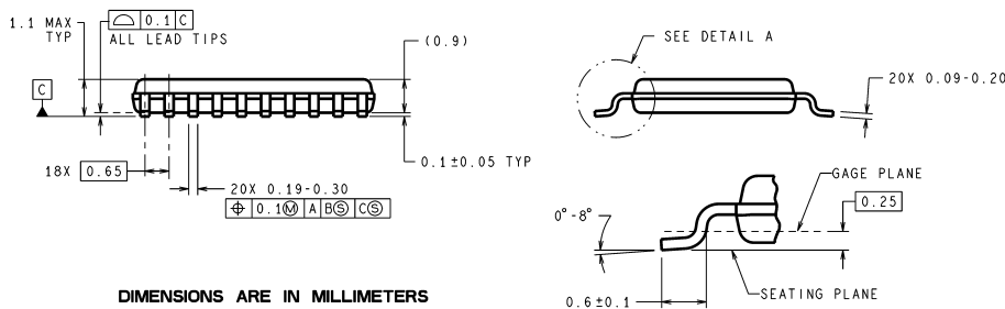
20-Lead Molded PKG, TSSOP, JEDEC, 4.4mm BODY WIDTH Order Number LM4863MT NS Package Number MTC20
