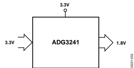
Figure 32. 3.3 V to 1.8 V Voltage Translation, \overline{SEL} = 0\text{ V}
