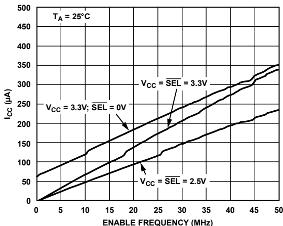
Figure 12. I_{CC} vs. Enable Frequency
