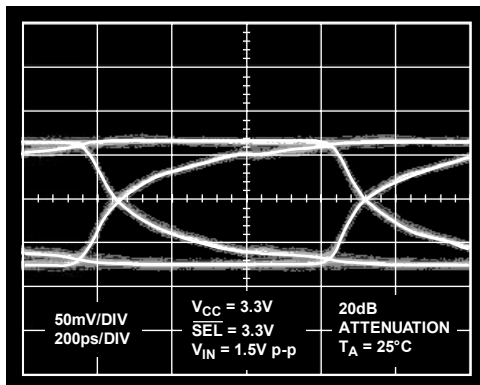
Figure 22. Eye Pattern; 1.5 Gbps, V_{CC} = 3.3V , PRBS 31
