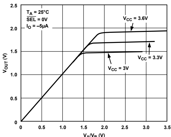
Figure 11. Pass Voltage vs. V_{CC}
