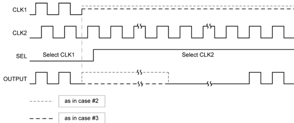
Timing Diagram 4
