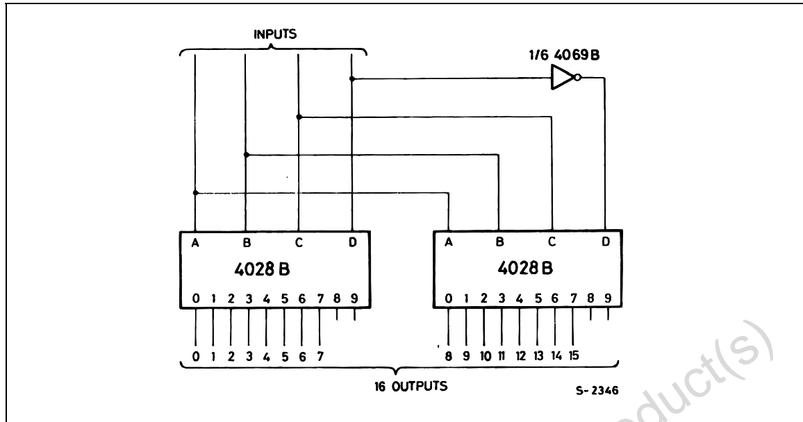
FIGURE 1 : CODE CONVERSION CIRCUIT
