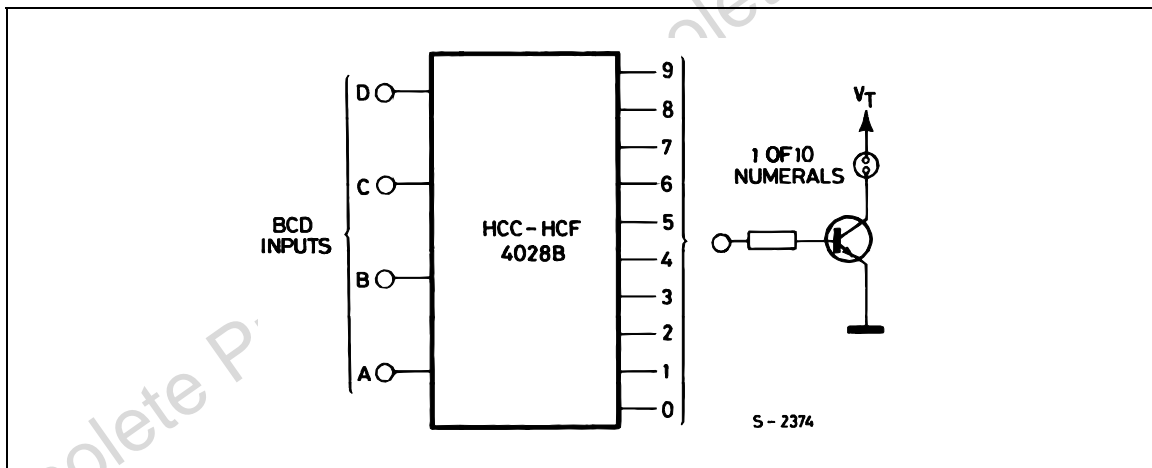
FIGURE 4 : NEON READOUT (NIXIE TUBE) DISPLAY APPLICATION
