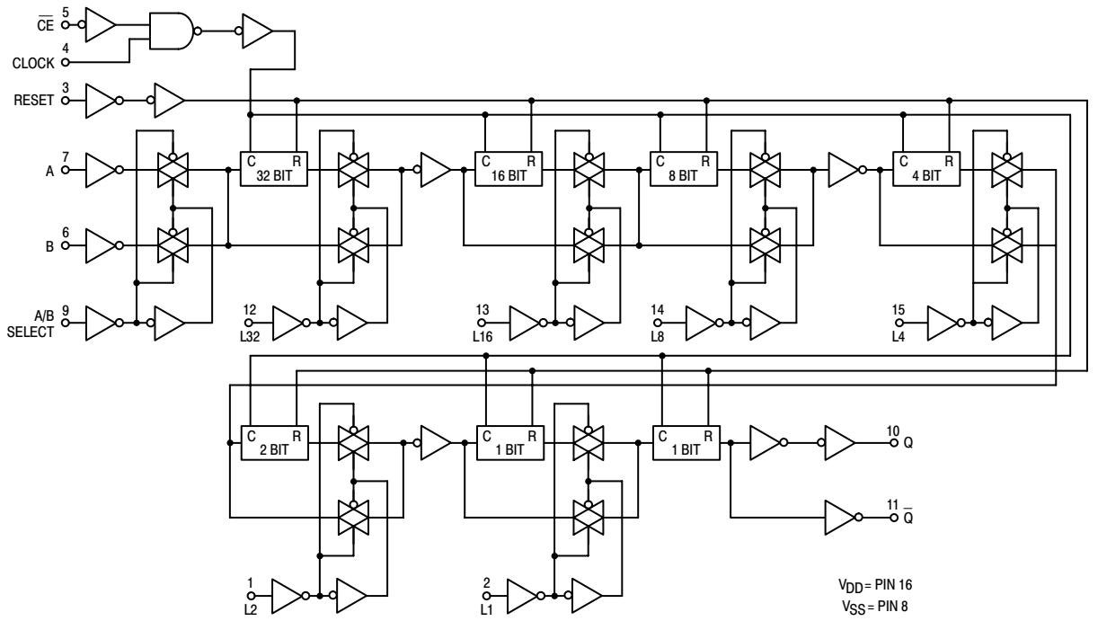
Figure 1. Logic Diagram
