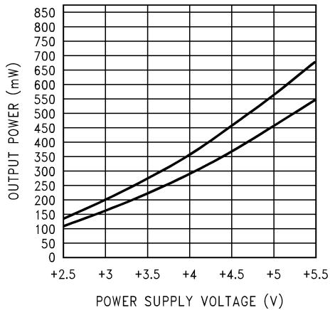
Output Power vs Power Supply Voltage
