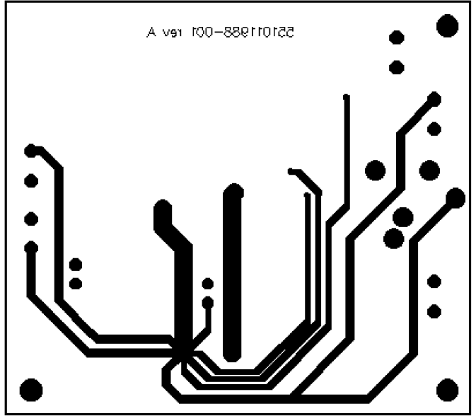
FIGURE 4. Recommended MM PC Board Layout: Bottom-Side Layout
