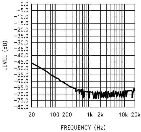
Input terminated with 10\Omega
