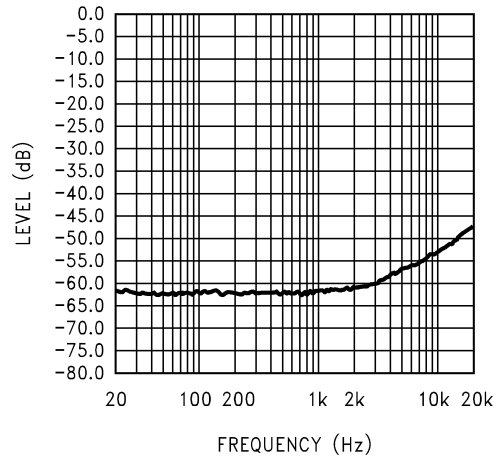
Input Floating
