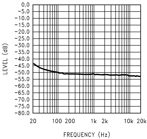
Input terminated with 10\Omega
