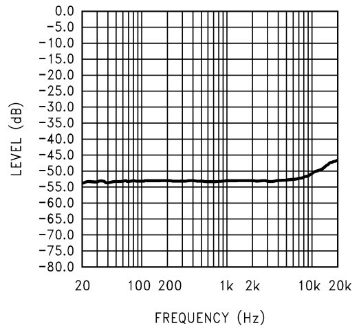
Input Floating
