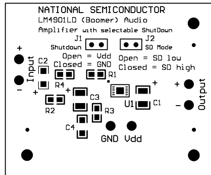
Silk Screen
