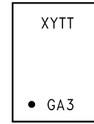
Top View XY - Date Code TT - Die Traceability G - Boomer Family A3 - LM4902LD
