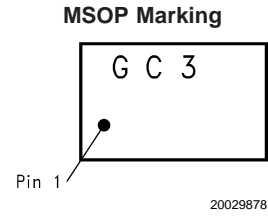
Top View G - Boomer Family C3 - LM4902MM
