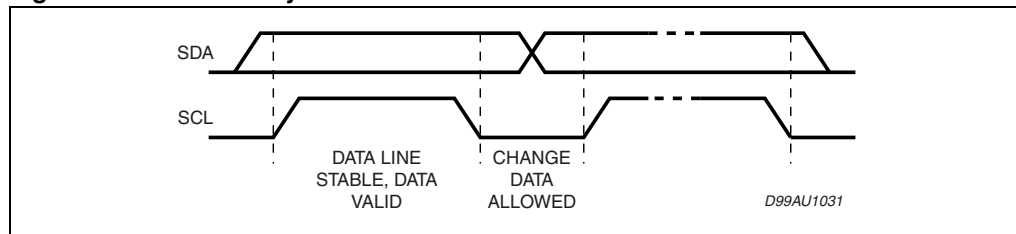
Figure 29. Data validity on the I 2 C bus
