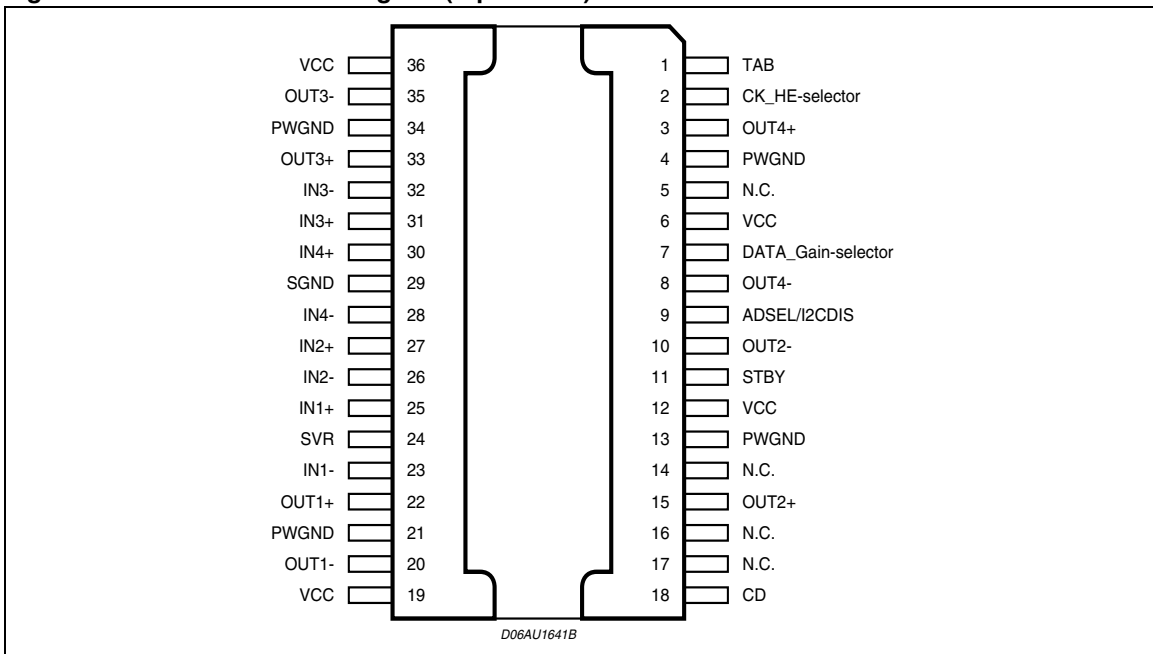
Figure 3. Pins connection diagram (top of view)
