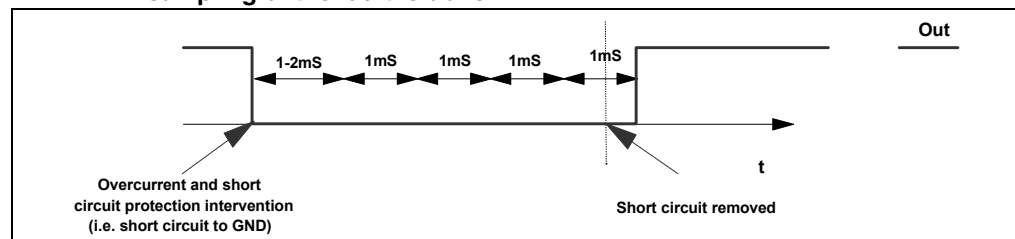
Figure 12. Restart timing with diagnostic enable (permanent)
