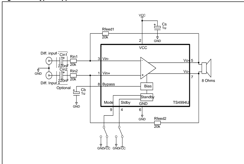
Figure 1. Typical application
