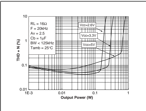
Figure 66. THD+N vs. output power
