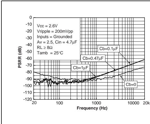
Figure 26. PSRR vs. frequency
