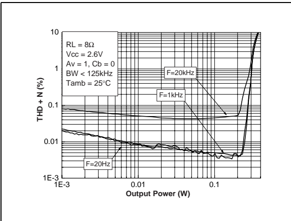
Figure 80. THD+N vs. output power
