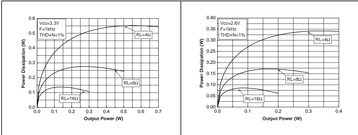
Figure 8. Power dissipation vs. output power Figure 9. Power dissipation vs. output power
