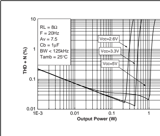
Figure 46. THD+N vs. output power
