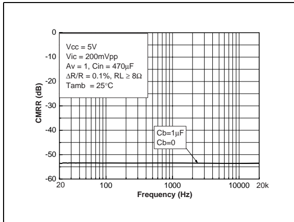
Figure 94. CMRR vs. frequency (worst case conditions)
