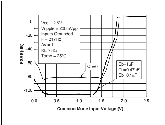
Figure 32. PSRR vs. common mode input voltage
