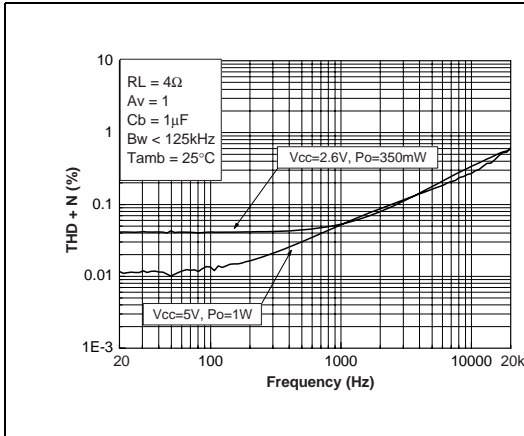
Figure 70. THD+N vs. frequency
