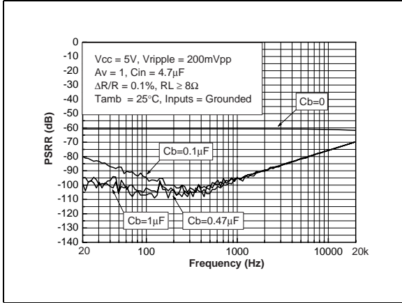
Figure 89. PSRR vs. frequency (worst case conditions)
