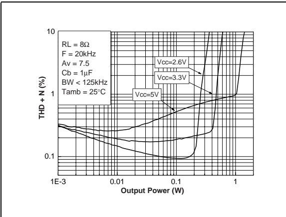
Figure 64. THD+N vs. output power
