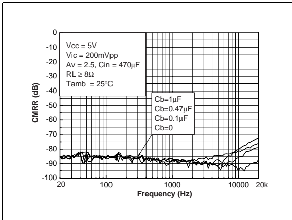
Figure 36. CMRR vs. frequency
