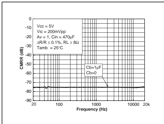
Figure 96. CMRR vs. frequency with random selection condition
