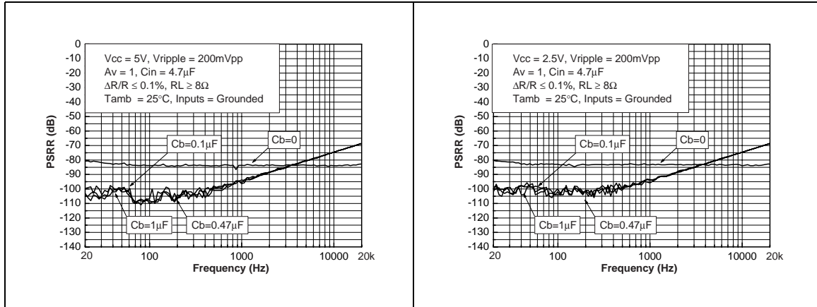
Figure 92. PSRR vs. frequency with random choice condition
