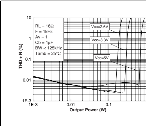
Figure 56. THD+N vs. output power
