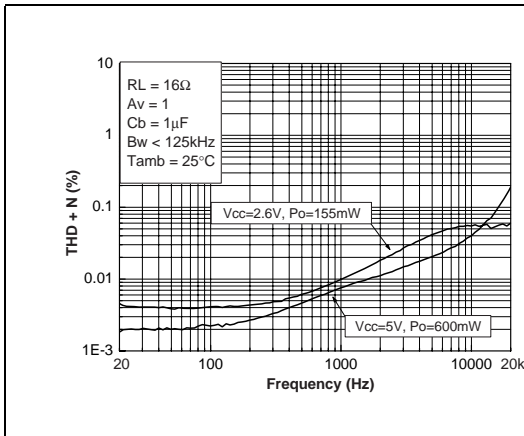
Figure 72. THD+N vs. frequency
