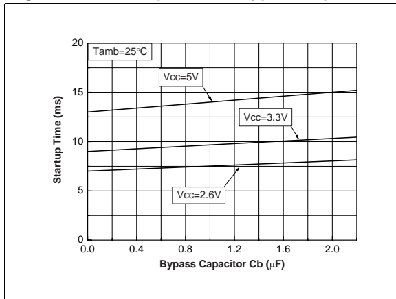
Figure 88. Startup time vs. bypass capacitor
