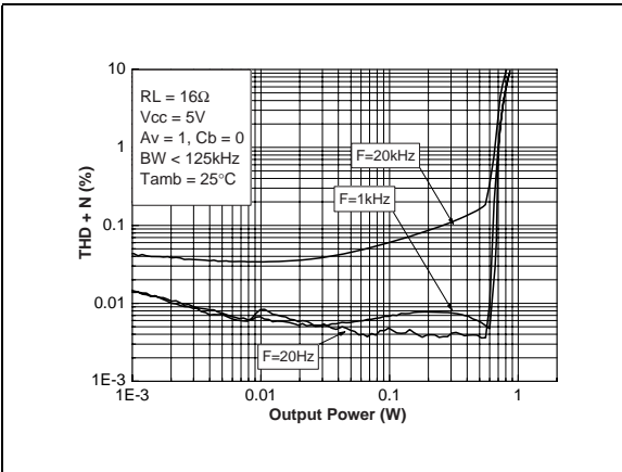
Figure 82. THD+N vs. output power
