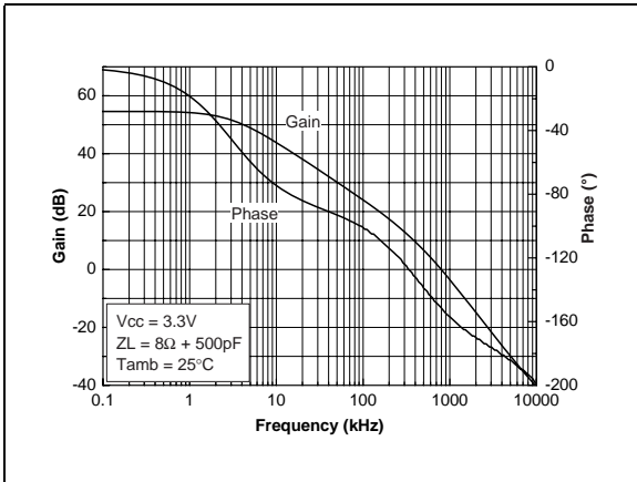
Figure 16. Open loop gain vs. frequency
