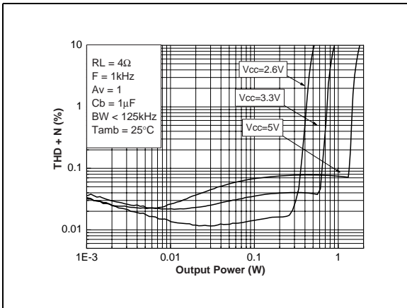
Figure 52. THD+N vs. output power
