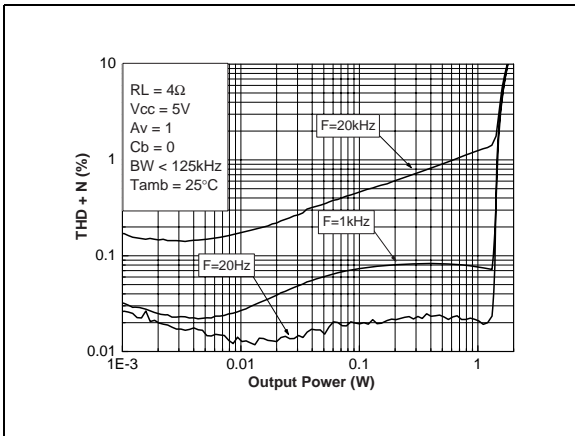
Figure 76. THD+N vs. output power
