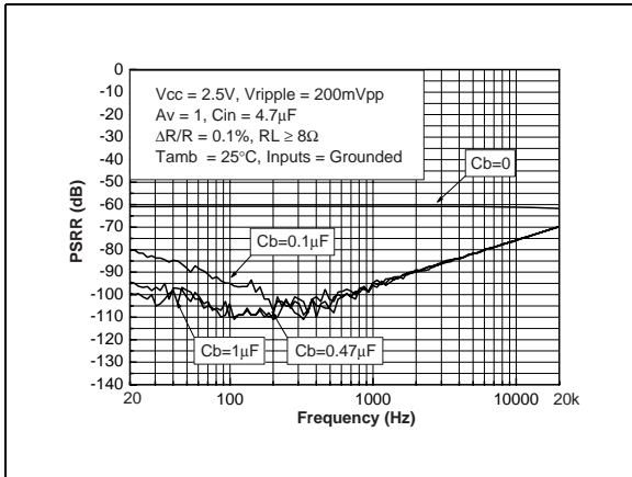
Figure 91. PSRR vs. frequency (worst case conditions)
