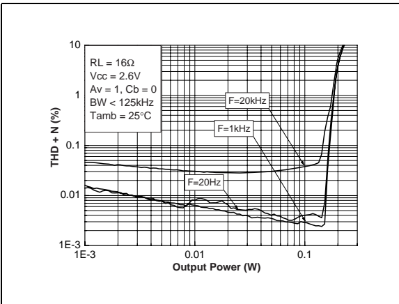
Figure 84. THD+N vs. output power
