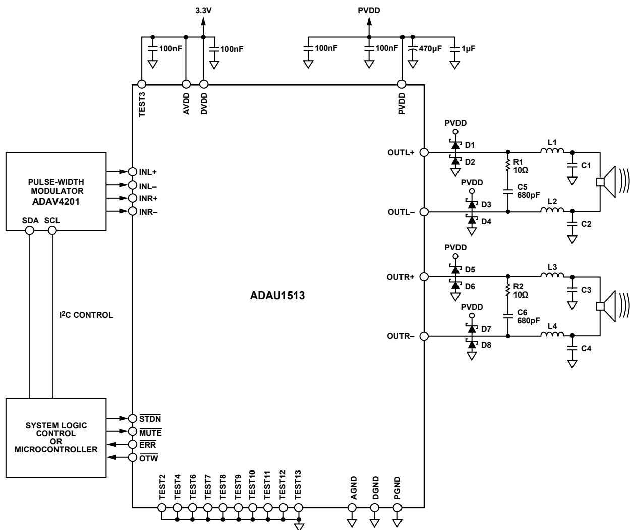
Figure 31. Application Schematic
