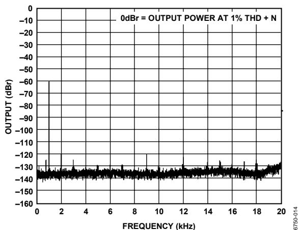
Figure 15. FFT, 60 dBFS, 15 V, 8 Ω
