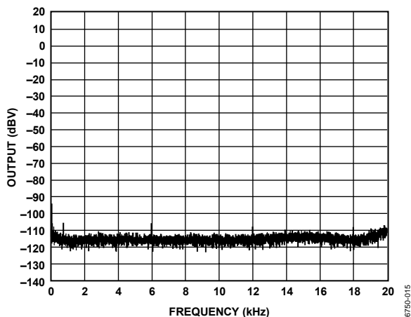
Figure 16. FFT Dither, 15 V, 8 Ω
