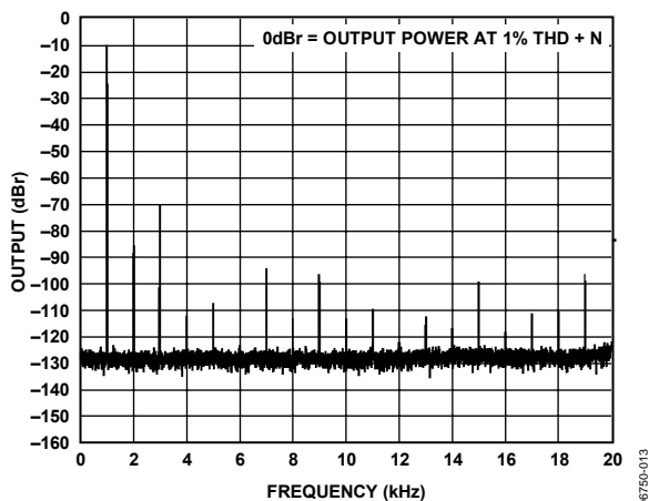
Figure 14. FFT, 1 W, 15 V, 8 Ω
