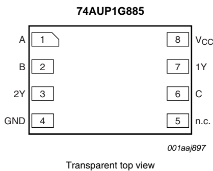
Fig 4. Pin configuration SOT996-2
