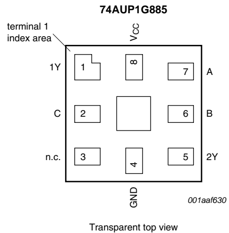
Fig 5. Pin configuration SOT902-1
