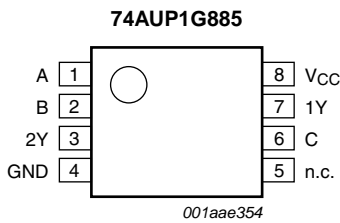
Fig 2. Pin configuration SOT765-1
