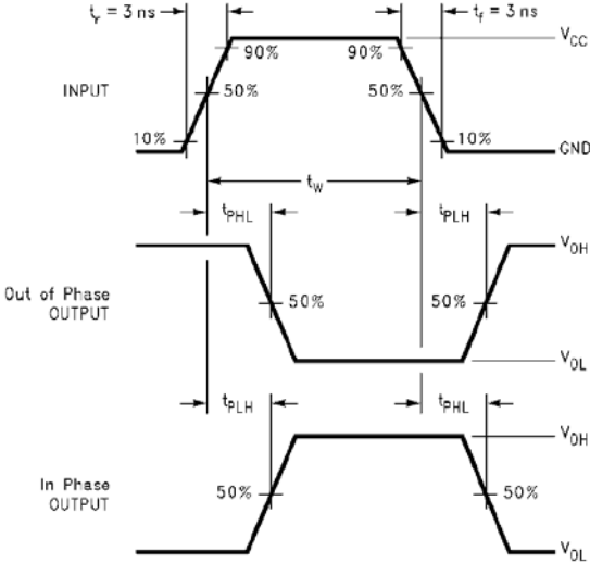
Figure 16. AC Waveforms
