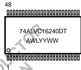
TSSOP-48 DT SUFFIX CASE 1201
