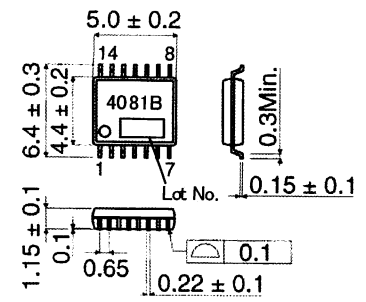
BU4081BFV(SSOP-B14)(UNIT:[mm])
