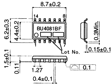
BU4081BF(SOP14)(UNIT:[mm])
