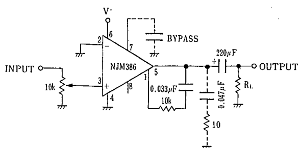
Amplifier 2
