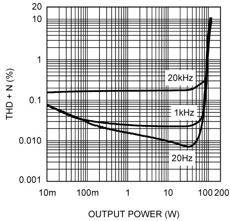
THD+N vs Output Power \pm 24\text{V} , All Chs in Parallel Mode (Note18), R_L = 2\Omega , 80kHz BW
