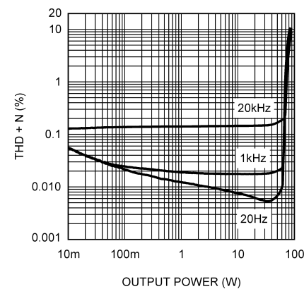
THD+N vs Output Power \pm 28V , Chs 1&3 in Parallel Mode (Note18), R_L = 4\Omega , 80kHz BW
