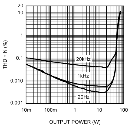
THD+N vs Output Power \pm 20V , Chs 1&3 in Bridge Mode (Note17), R_L = 8\Omega , 80kHz BW
