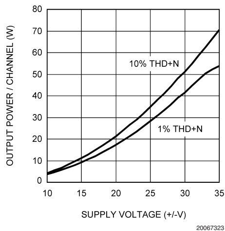
Output Power/Channel vs Supply Voltage f = 1\text{kHz} , R_L = 8\Omega , 80kHz BW
