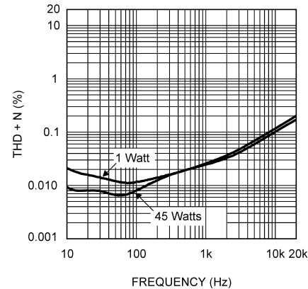
THD+N vs Frequency \pm 24V , P_{OUT} = 1W & 45W , All Chs in Parallel Mode (Note18), R_L = 2\Omega , 80kHz BW
