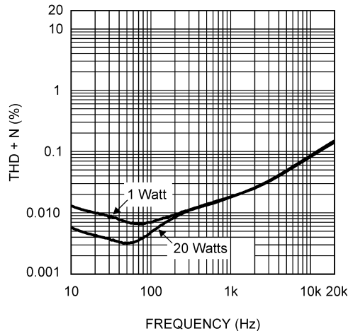
THD+N vs Frequency \pm 28V , P_{OUT} = 1W \text{ \& } 20W/\text{Channel} R_L = 8\Omega , 80kHz BW
