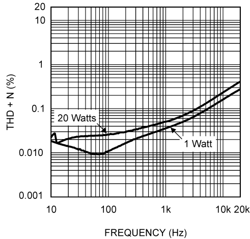
THD+N vs Frequency \pm 20V , P_{OUT} = 1W \text{ \& } 20W/\text{Channel} R_L = 4\Omega , 80kHz BW
