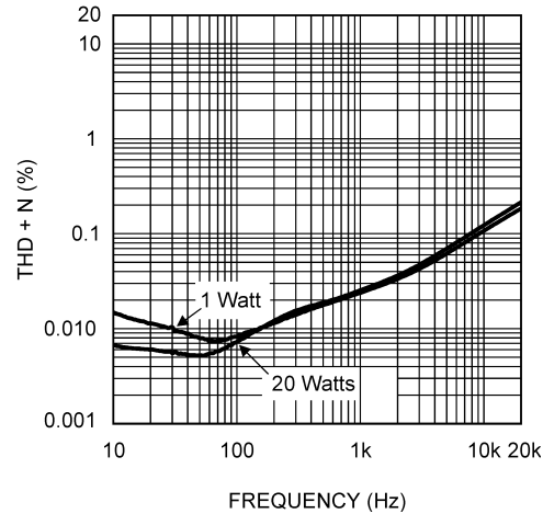
THD+N vs Frequency \pm 24V , P_{OUT} = 1W \text{ \& } 20W/\text{Channel} R_L = 6\Omega , 80kHz BW
