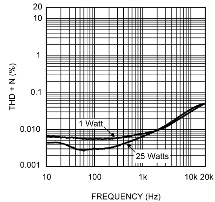
THD+N vs Frequency \pm 20V , P_{OUT} = 1W & 25W , Chs 1&3 in Bridge Mode (Note17), R_L = 8\Omega , 80kHz BW
