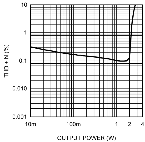
THD+N vs Output Power V_{DD} = 5V, R_L = 3\Omega, f = 1kHz
