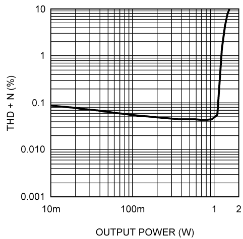
THD+N vs Output Power V_{DD} = 5V, R_L = 8\Omega, BTL, f = 1kHz
