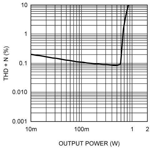
THD+N vs Output Power V_{DD} = 3V, R_L = 4\Omega, f = 1kHz
