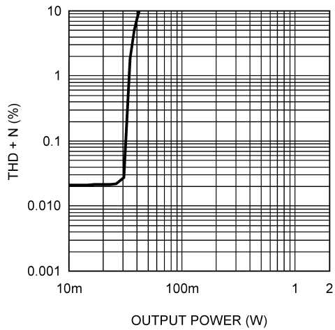
THD+N vs Output Power V_{DD} = 3V, R_L = 32\Omega, SE, f = 1kHz
