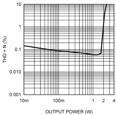
THD+N vs Output Power V_{DD} = 5V, R_L = 4\Omega, f = 1kHz
