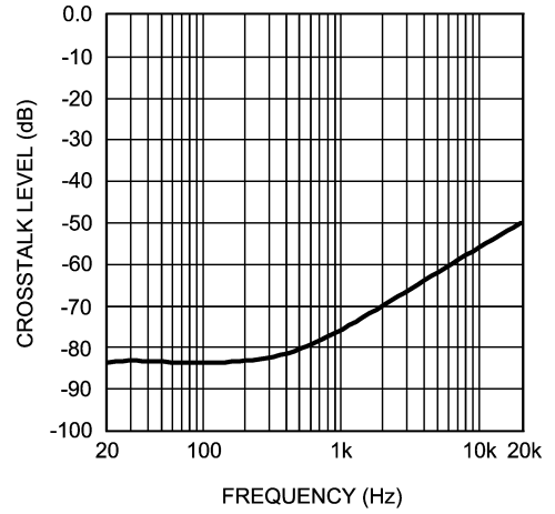
Crosstalk vs Frequency V_{DD} = 5V, R_L = 8\Omega, P_O = 1W
