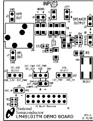
Silk Screen
