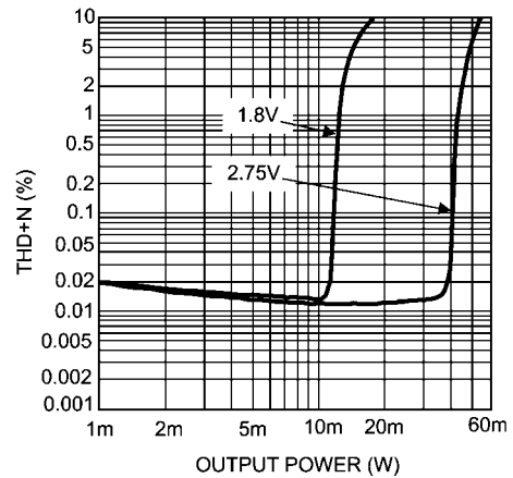
THD+N vs Output Power V_{DDLS} = 3.3V , V_{DDHP} = 1.8V & 2.75V , f = 1kHz , R_L = 32\Omega SE, Mode 8 (Left/Right), 80kHz BW
