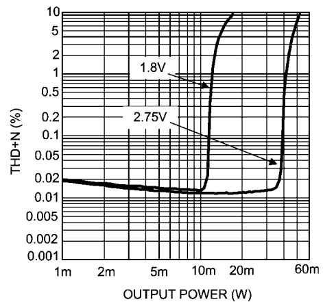
THD+N vs Output Power V_{DDLS} = 3.3V , V_{DDHP} = 1.8V & 2.75V , f = 1kHz , R_L = 32\Omega SE, Mode 10 (Left/Right), 80kHz BW
