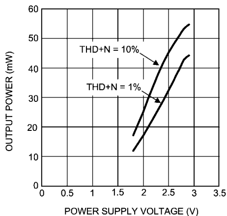
Output Power vs Supply Voltage ( V_{DDLS} ) V_{DDLS} = 3.3V , R_L = 32\Omega SE, Mode 4
