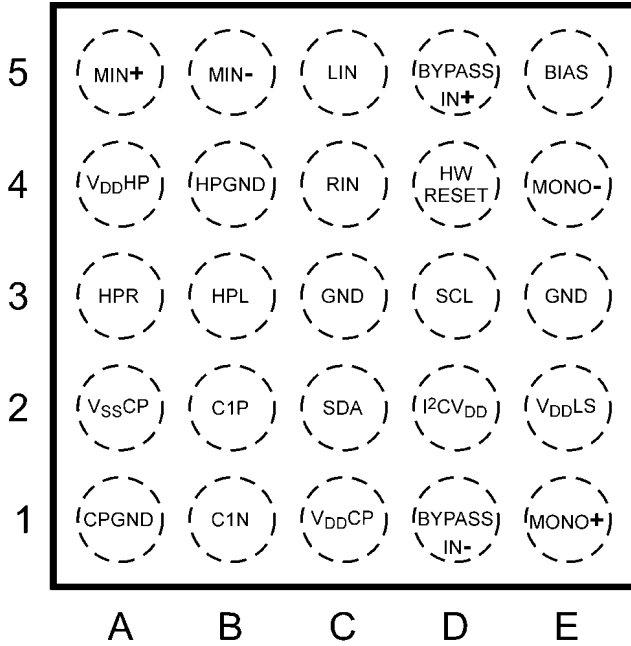
25 Bump micro SMD Package
