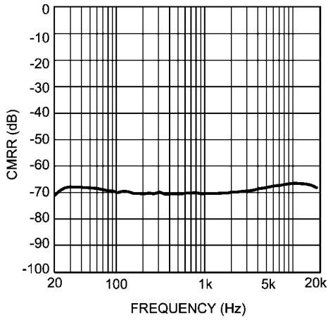
CMRR vs Frequency V_{DD} = 3.2V, Z_L = 1\mu F + 20\Omega V_{IN} = 100mV_{P-P}
