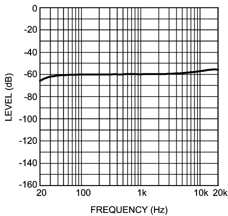
PSRR vs Frequency V_{DD} = 4.2V, R_L = 16\Omega
