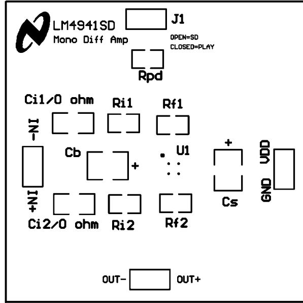
Recommended LLP Board Layout: Top Overlay 20170375
