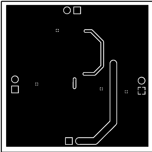
Recommended LLP Board Layout: Bottom Layer 20170377
