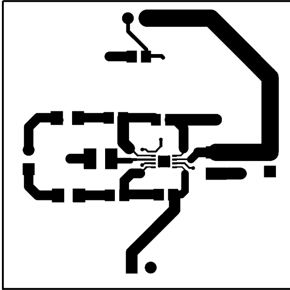
Recommended LLP Board Layout: Top Layer 20170376
