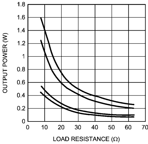
Output Power vs Load Resistance Top- V_{DD} = 5V , 10% THD+N, Topmid- V_{DD} = 5V , 1% THD+N Bot- V_{DD} = 3V , 10% THD+N, Botmid- V_{DD} = 3V , 1% THD+N
