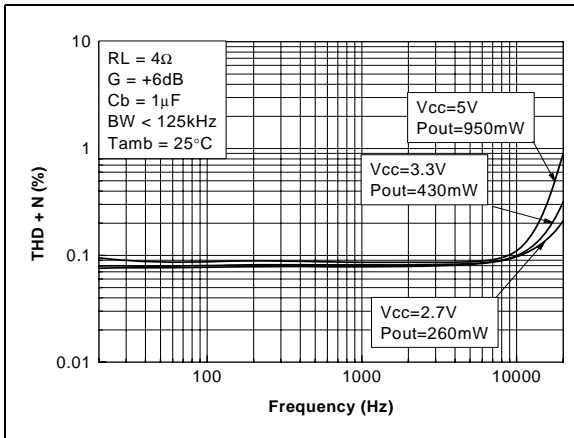
Figure 16. THD+N vs. frequency
