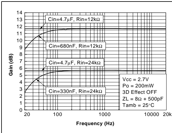
Figure 56. Frequency response
