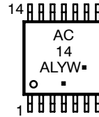
TSSOP-14
