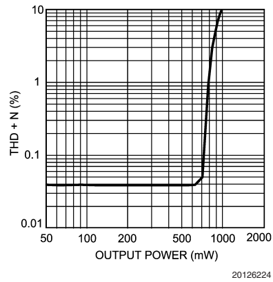
THD+N vs Output Power V_{DD} = 4.2V, A_V = 26dB, R_L = 16\Omega
