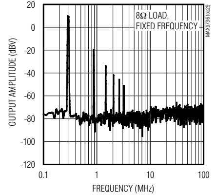
WIDEBAND OUTPUT SPECTRUM
