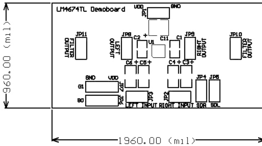
Top Silkscreen
