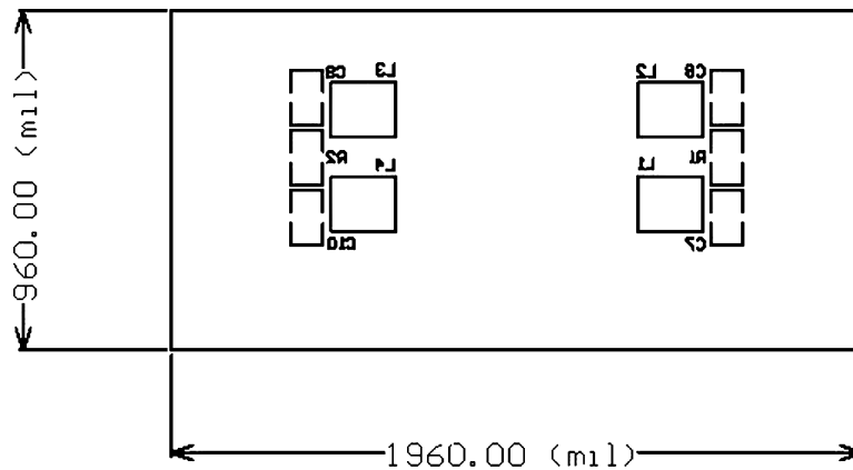
Bottom Silkscreen
