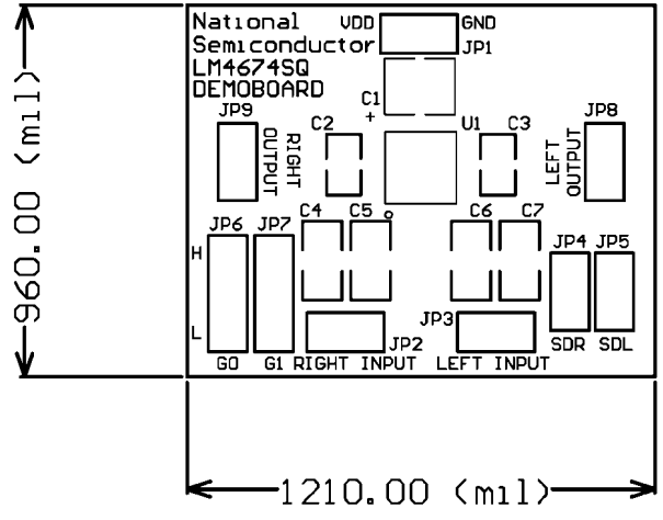
Top Silkscreen
