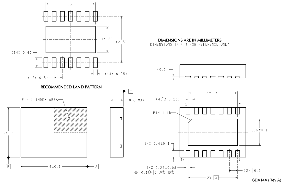
LLP Package Order Number LM4928SD NS Package Number SDA14A
