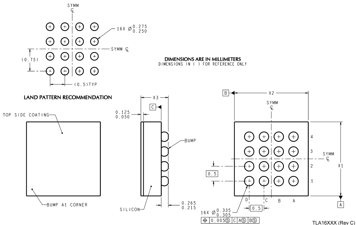
16-bump micro SMD Order Number LM4928TL NS Package Number TLA1611A X1 = 1.970±0.03, X2 = 1.970±0.03, X3 = 0.600±0.075
