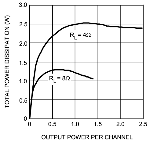
Power Dissipation vs Output Power V_{DD} = 5V
