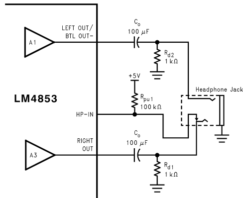
FIGURE 2. Headphone Control Circuit
