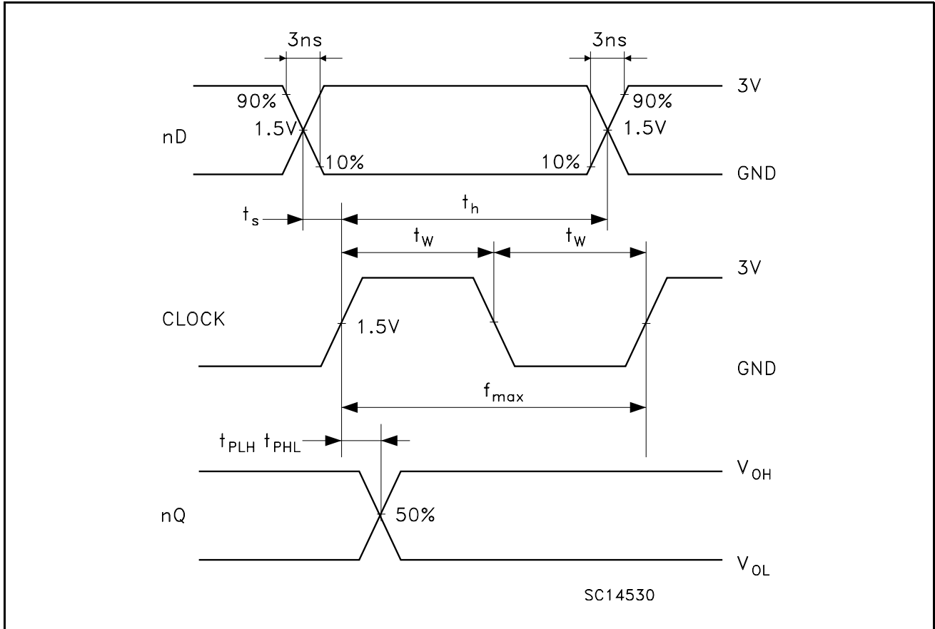
Figure 5: Waveform - Propagation Delays (f=1MHz; 50% duty cycle)
