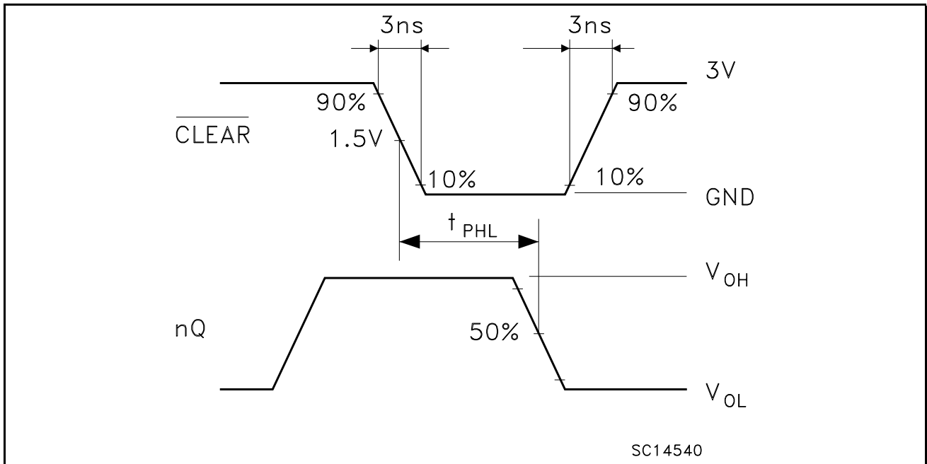
Figure 5: Waveform - Propagation Delays (f=1MHz; 50% duty cycle)
