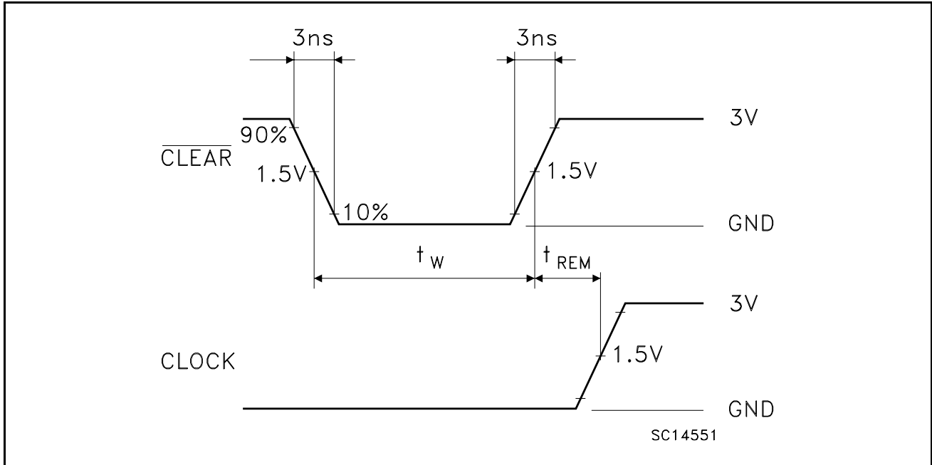
Figure 6: Waveform - Recovery Time ( f=1\text{MHz} ; 50% duty cycle)
