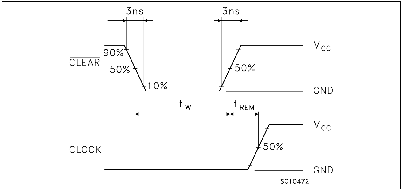
Figure 7: Waveform - Recovery Time ( f=1\text{MHz} ; 50% duty cycle)
