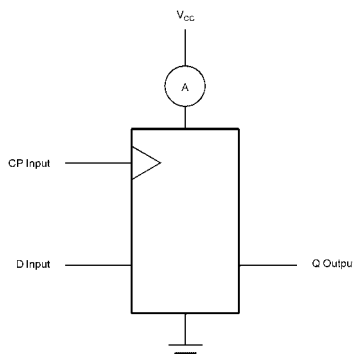
FIGURE 2. I_{CCD} Test Circuit
