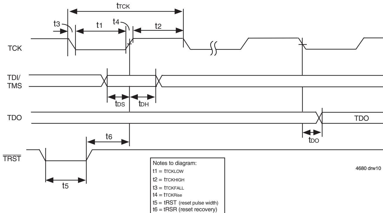
Figure 5. Standard JTAG Timing
