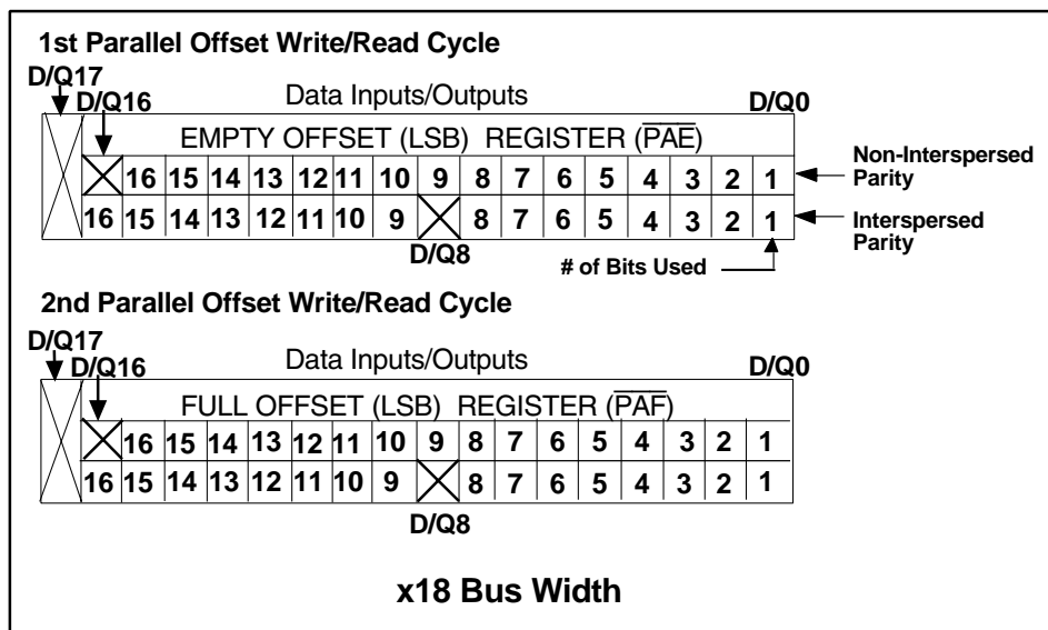
Figure 3. Programmable Flag Offset Programming Sequence (Continued)
