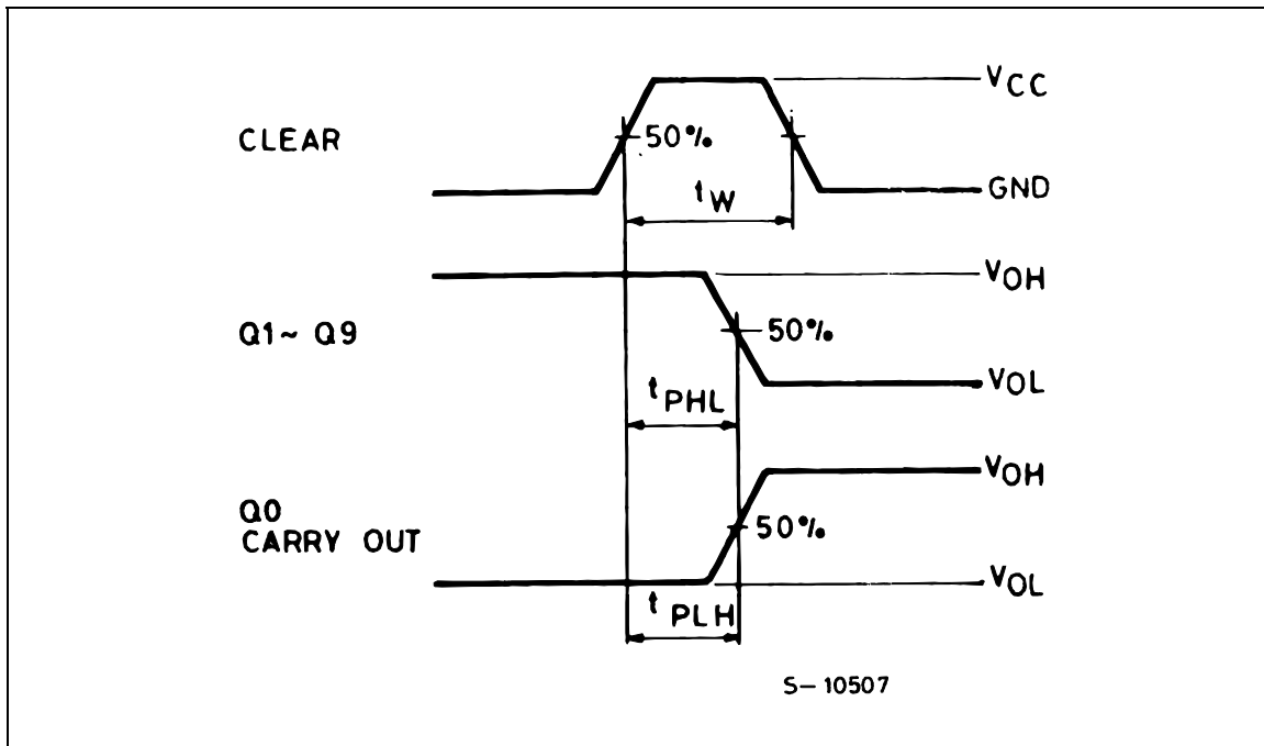
WAVEFORM 3 : MINIMUM PULSE WIDTH, PROPAGATION DELAY (f=1MHz; 50% duty cycle)
