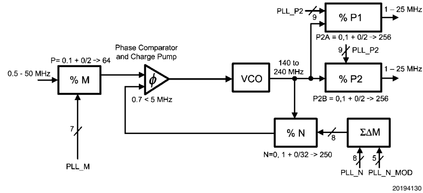
FIGURE 13. PLL1 Loop
