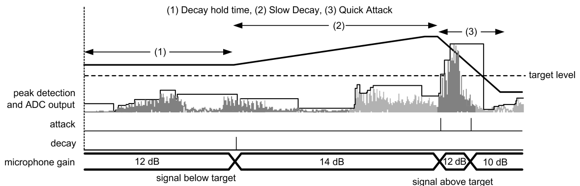
FIGURE 23. ALC Example
