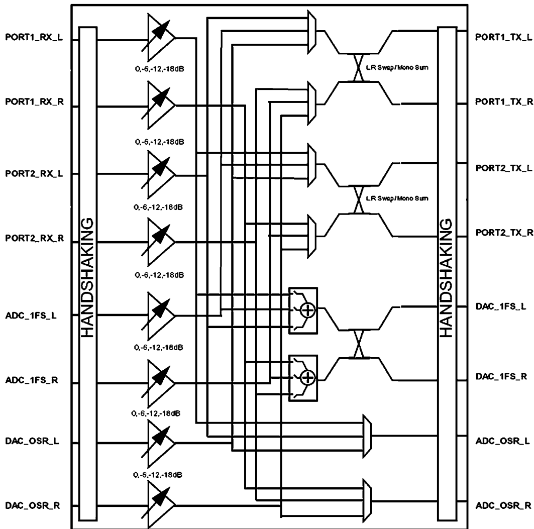
FIGURE 16. Digital Mixer
