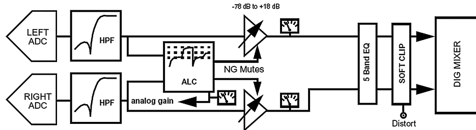
FIGURE 21. ADC DSP Effects Chain
