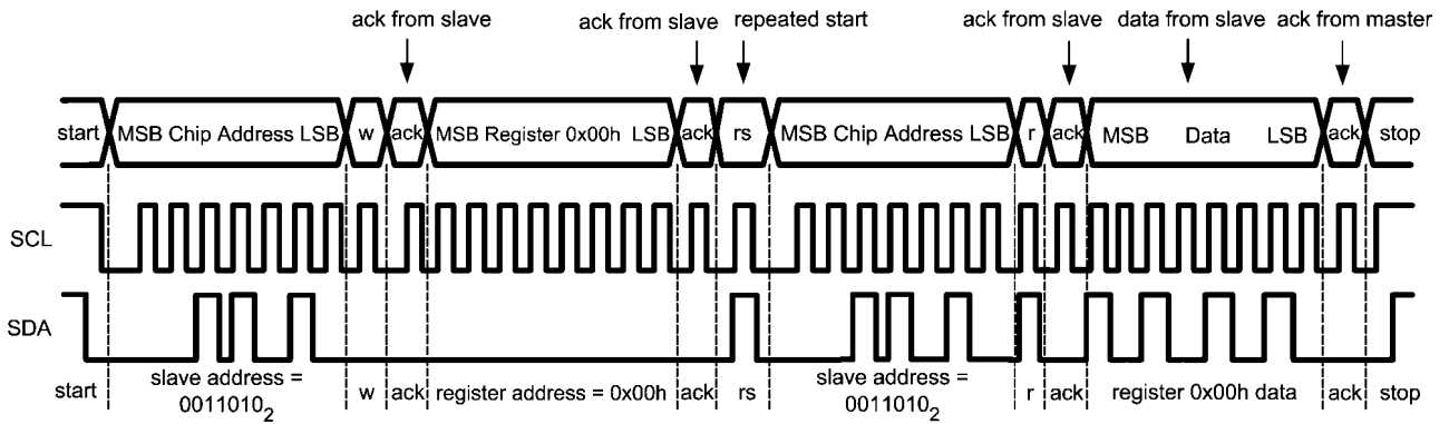
FIGURE 10. Example I 2 C Read Cycle
