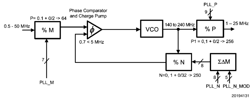
FIGURE 14. PLL2 Loop
