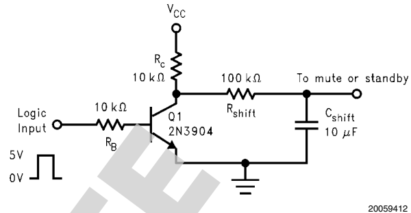
FIGURE 5. Level Shift Circuit
