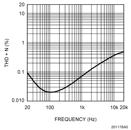
THD+N vs Frequency V_{DD} = 3V , R_L = 8\Omega , A_{V-SE} = 1V/V P_{OUT} = 50mW/Channel , 80kHz BW
