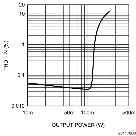
THD+N vs Output Power/Channel V_{DD} = 3V , R_L = 8\Omega , A_{V-SE} = 1V/V f = 1kHz , C_{OUT} = 220\mu F , 80kHz BW
