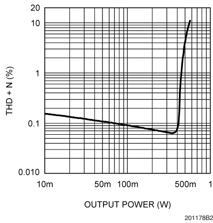
THD+N vs Output Power/Channel V_{DD} = 3V , R_L = 8\Omega , A_{V-SE} = 1V/V f = 1kHz , C_{OUT} = 220\mu F , 80kHz BW
