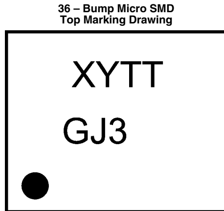
20202031 Top View XY — 2 Digit Date Code TT — Die Traceability G — Boomer Family J3 — LM4937RL
