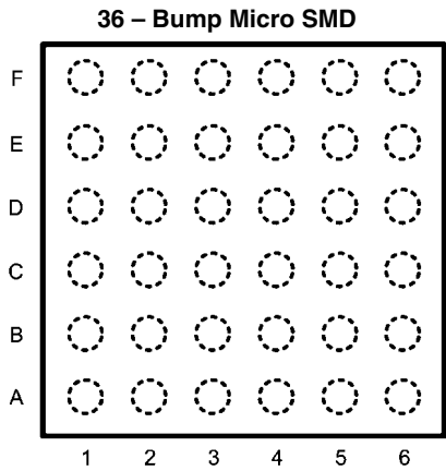
20202058 Top View (Bump Side Down) Order Number LM4937RL See NS Package Number RLA36LVA
