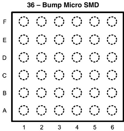
20202058 Top View (Bump Side Down) Order Number LM4937TL See NS Package Number TLA36LVA
