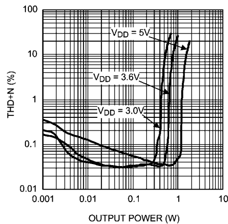
THD+N vs Output Power A_V = 6\text{dB} , R_L = 8\Omega , f = 1\text{kHz} Analog Input, Speaker Mode
