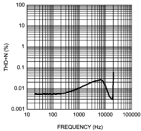
THD+N vs Frequency HPV_{DD} = 2.5V, P_{OUT} = 25mW, R_L = 32\Omega DAC Input, Internal Reference, Headphone Mode
