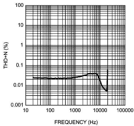
THD+N vs Frequency HPV_{DD} = 2.5V, P_{OUT} = 25mW, R_L = 16\Omega DAC Input, External Reference, Headphone Mode
