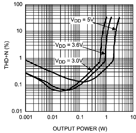
THD+N vs Output Power A_V = 12\text{dB} , R_L = 4\Omega , f = 1\text{kHz} DAC Input, External Reference, Speaker Mode
