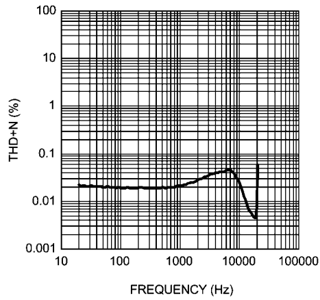
THD+N vs Frequency HPV_{DD} = 2.5V, P_{OUT} = 25mW, R_L = 16\Omega DAC Input, Internal Reference, Headphone Mode
