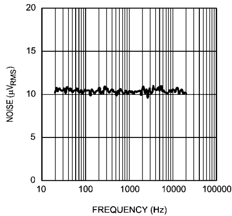
Output Noise vs Frequency HPV_{DD} = 2.5\text{V} , R_L = 32\Omega Analog Input, Headphone Mode
