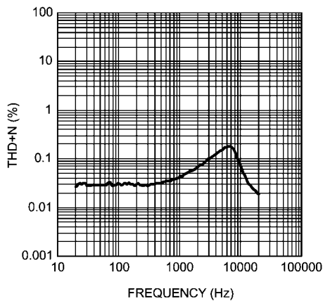
THD+N vs Frequency V_{DD} = 3.0V , P_{OUT} = 100mW , R_L = 4\Omega Analog Input, Speaker Mode
