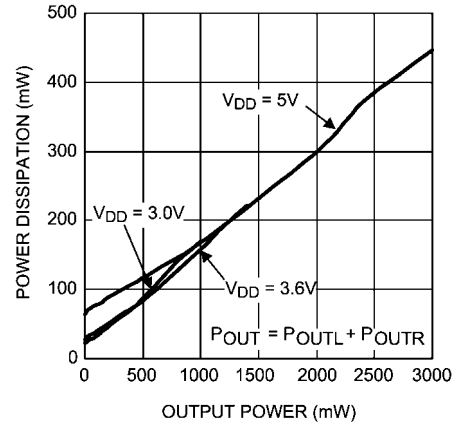
Power Dissipation vs Output Power R_L = 8\Omega, f = 1\text{kHz}, \text{Speaker Mode}
