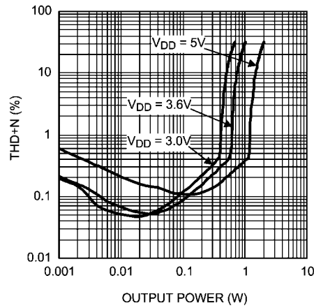
THD+N vs Output Power A_V = 12\text{dB} , R_L = 8\Omega , f = 1\text{kHz} DAC Input, External Reference, Speaker Mode
