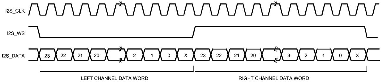
FIGURE 6. I 2 S Left Justified Input Format
