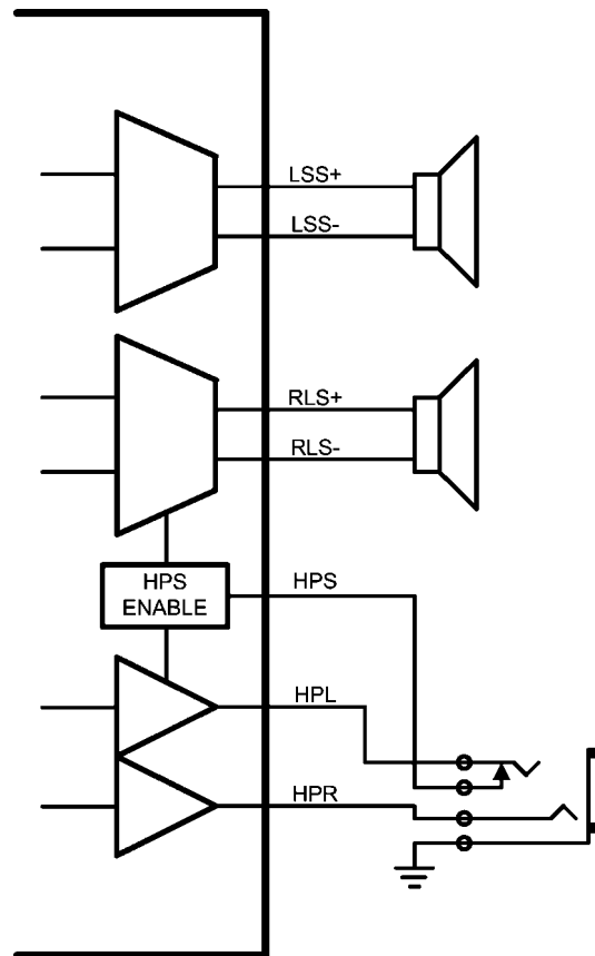
FIGURE 8. HPS Connection
