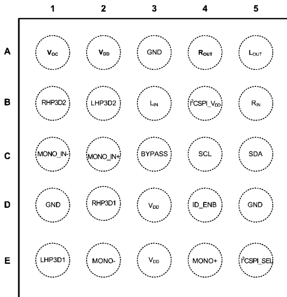
25 Bump micro SMD Package
