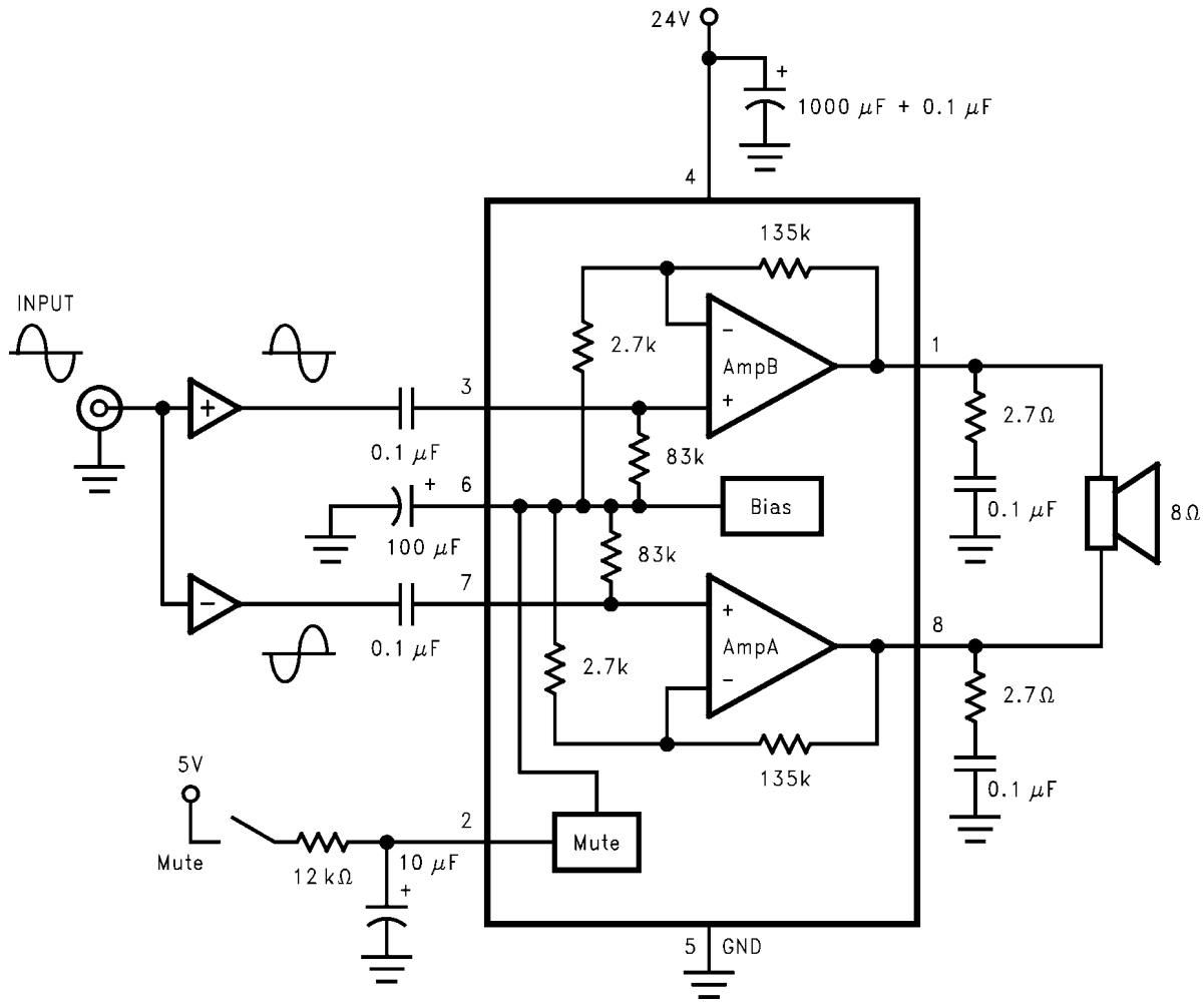
FIGURE 4. Bridge-Mode Application
