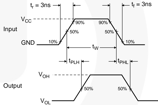
Figure 6. AC Waveforms
