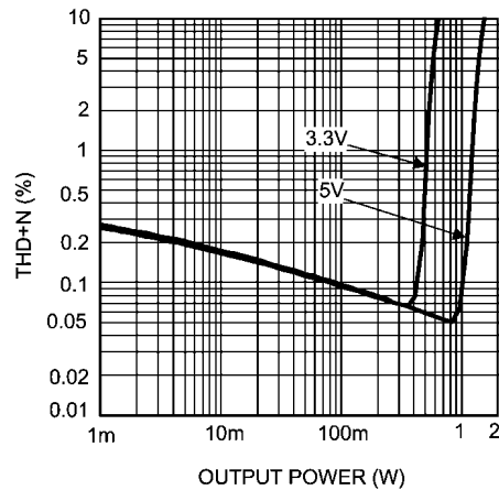
THD+N vs Output Power V_{DD} = 3.3V \text{ \& } 5V, R_L = 8\Omega, f = 1kHz Mode 5, 80kHz BW
