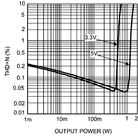
THD+N vs Output Power V_{DD} = 3.3V \text{ \& } 5V, R_L = 8\Omega \text{ BTL}, f = 1kHz Mode 2, 80kHz BW
