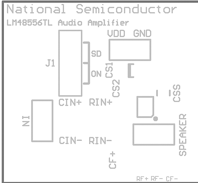
FIGURE 4: Top Overlay
