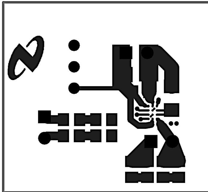
FIGURE 5: Top Layer
