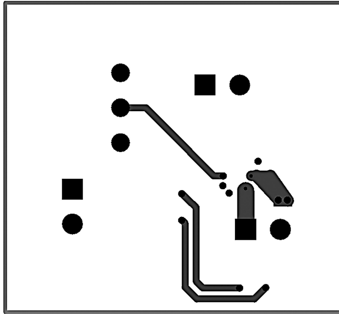
FIGURE 6: Mid Layer 1
