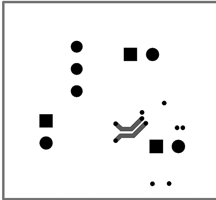
FIGURE 7: Mid Layer 2
