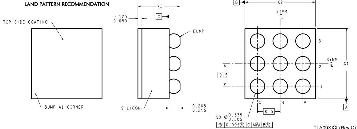
9-Bump micro SMD Order Number LM4890ITL, LM4890ITLX NS Package Number TLA09AAA X1 = 1.514±0.03 X2 = 1.514±0.03 X3 = 0.600±0.075
