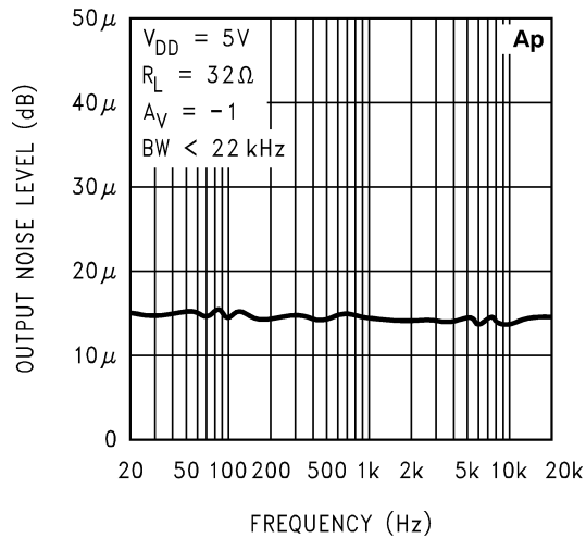
Noise Floor
